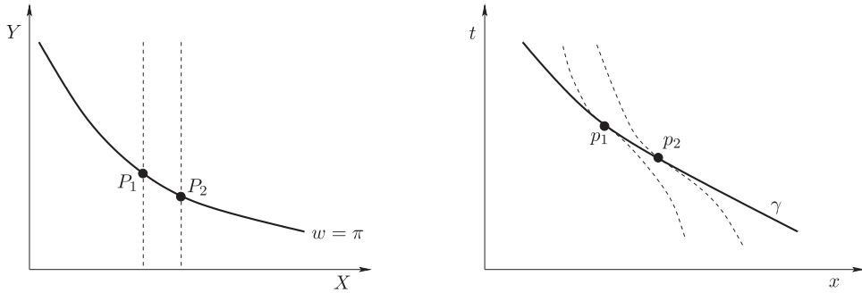
Figure 4: Left: a singular curve where w = \pi , in the X - Y plane. Vertical lines where X = \text{constant} correspond to characteristic curves of the wave equation (1.1), where \dot{x} = -c(u) . Right: the images of these curves in the x - t plane, under the map \Lambda at (2.26). The singular curve \gamma is an envelope of characteristic curves, which cross it tangentially.
