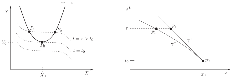
Figure 5: Left: the equation w(X, Y) = \pi implicitly defines a function Y(X) with a strict local minimum at X_0 . Under generic conditions, Y''(X_0) > 0 . The dotted curves where t(X, Y) = \tau have 0, 1, or 2 intersections respectively, if \tau < t_0 , \tau = t_0 , or \tau > t_0 . Right: the image of the curve \{w = \pi\} under the map \Lambda in (2.26) consists of two singular curves \gamma^-, \gamma^+ starting at the point p_0 = (x_0, t_0) . For \tau > t_0 , the distance between these two curves is \gamma^+(\tau) - \gamma^-(\tau) = \mathcal{O}(1) \cdot (\tau - t_0)^{5/2} .
