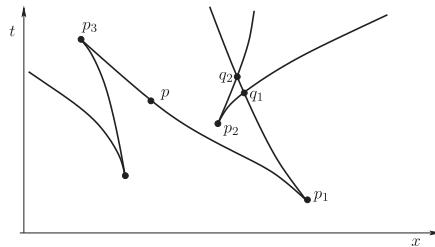
Figure 3: The images of the level sets \{w = \pi\} and \{z = \pi\} in Figure 2, under the map \Lambda : (X, Y) \mapsto (x(X, Y), t(X, Y)) . In the x - t plane, these represents the curves where u = u(x, t) is not differentiable. A generic solution of (1.1) with smooth initial data remains smooth outside finitely many singular points and finitely many singular curves, where u_x \rightarrow \pm\infty . Here p_1, p_2, p_3 are singular points where two new singular curves originate, or two singular curves merge and disappear. At the points q_1, q_2 a forward and a backward singular curve cross each other.
