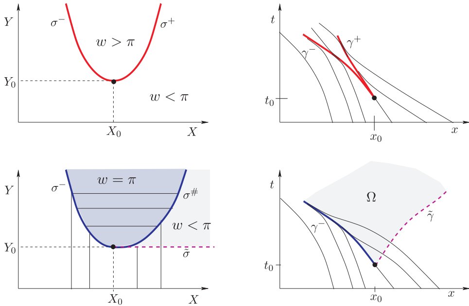
Figure 6: The positions of the singularities in the X - Y plane and in the x - t plane. This refers to a point where a new singularity is formed, in the first family (i.e., for backward moving waves). Above: a conservative solution. Below: a dissipative solution. Notice that the entire region between the curves \sigma^- and \sigma^\# is mapped onto the single curve \gamma^- . Indeed, horizontal segments in the X - Y plane are mapped into a single point. In the x - t plane, the two solutions differ only on the set \Omega , bounded by the characteristic curves \gamma^- (the image of both \sigma^- and \sigma^\# ) and \tilde{\gamma} (the image of the line \tilde{\sigma} ).
