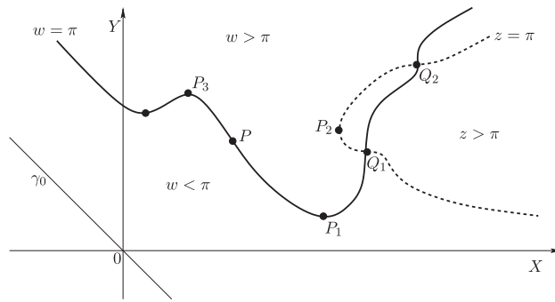
Figure 2: Two level sets \{w = \pi\} and \{z = \pi\} , in a generic conservative solution of (2.9)–(2.11). Here P is a singular point of Type 1, while P_1, P_2, P_3 are points of Type 2, and Q_1, Q_2 are points of Type 3. Notice that at P_1 , structural stability requires that the function Y(X) implicitly defined by w(X, Y(X)) = \pi has strictly positive second derivative. At the points Q_1, Q_2 , by (2.10) one has w_Y = z_X = 0 . Hence the two curves \{w = \pi\} and \{z = \pi\} have a perpendicular intersection.
