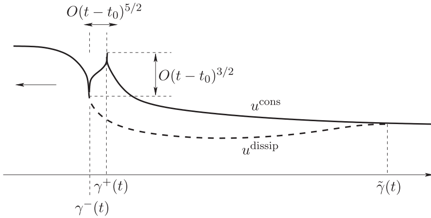
Figure 7: Comparing a conservative and a dissipative solution, at a time t > t_0 , after a singularity has appeared. The conservative solution has two strong singularities at \gamma^-(t) < \gamma^+(t) , while the dissipative solution has a strong singularity at \gamma^-(t) and a weak singularity at \tilde{\gamma}(t) . The two solutions coincide for x \leq \gamma^-(t) and for x \geq \tilde{\gamma}(t) .
