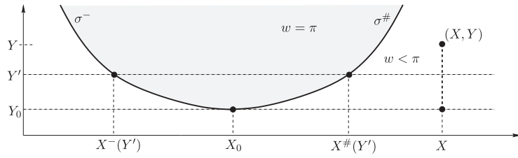
Figure 8: Estimating the values of a dissipative solution near a singularity. Notice that the functions x, t, u are constant on every horizontal segment contained in the shaded region where w = \pi .
