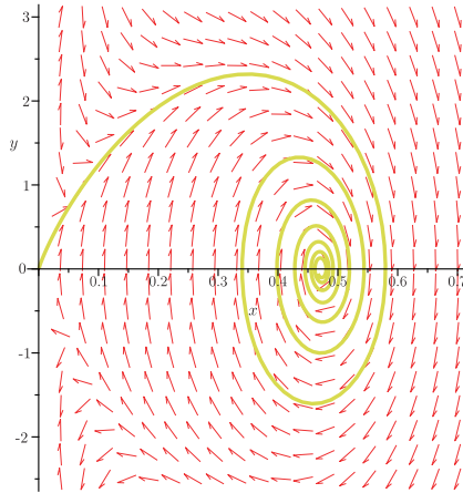
Figure 1: Case n = 200 , p = 2 , v_\infty = 0.4723 \dots .
