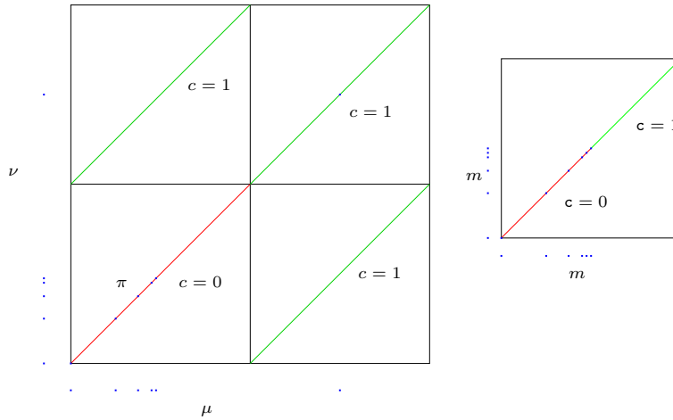
Figure 4. The cost of Example 6.6. Outside the diagonal segments the cost is +\infty .
