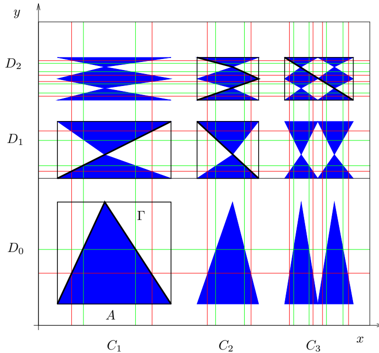
Figure 2. The set where A should be contained in order to have that A' is a subset of the standard order \leq on [0, 1] . The bold curves are the limbs of \Gamma , and two axial path are represented.
