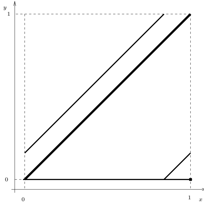
Figure 8. The cost function considered in Point (d) at Page 450.
