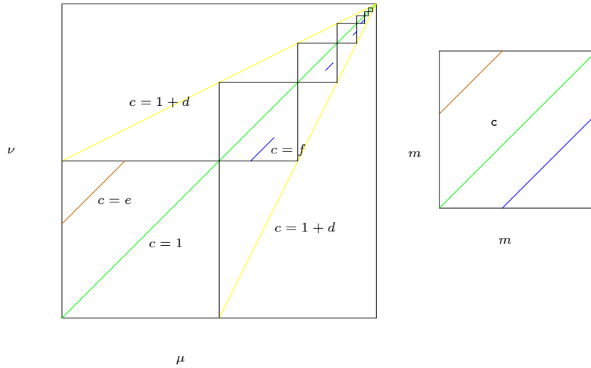
Figure 6. The cost of Example 6.8.
