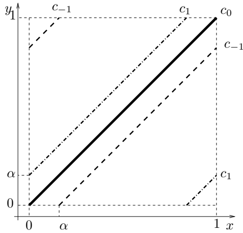
(a) When \alpha \notin \mathbb{Q} , the cycle decomposition of the plan \pi = (\text{Id}, \text{Id})_{\#} \mathcal{L}^1 gives only a consistent disintegration (Ex. 6.1).
